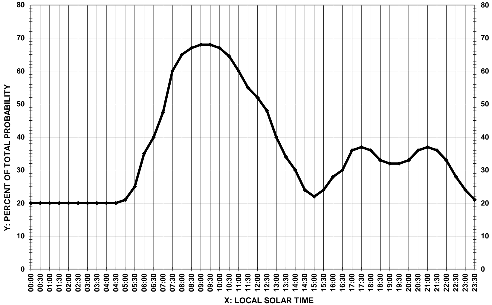
BASELINE 1-HOP RELATIVE PROBABILITY DIURNAL MODEL OF Es (Based on the work of E.K. Smith in Davies, 1990) and (Extreme Multi-Hop 50 MHz Es, Kennedy 2010)
